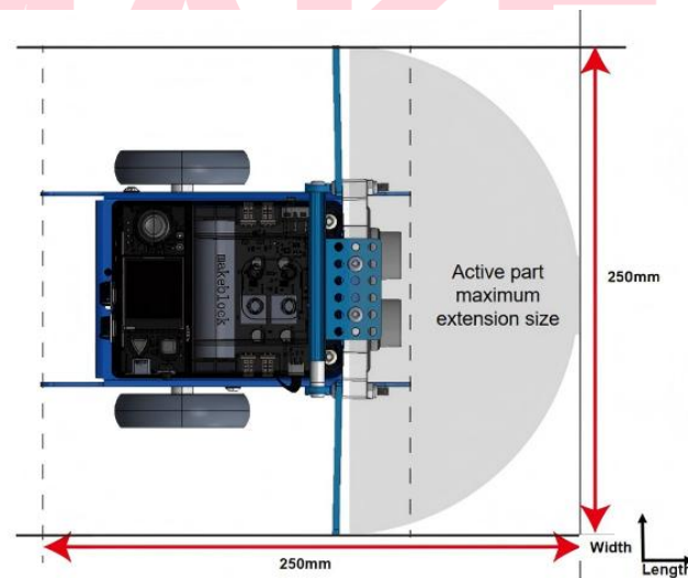
Fig. 5 .1-1 Maximum extension state (Top View)
